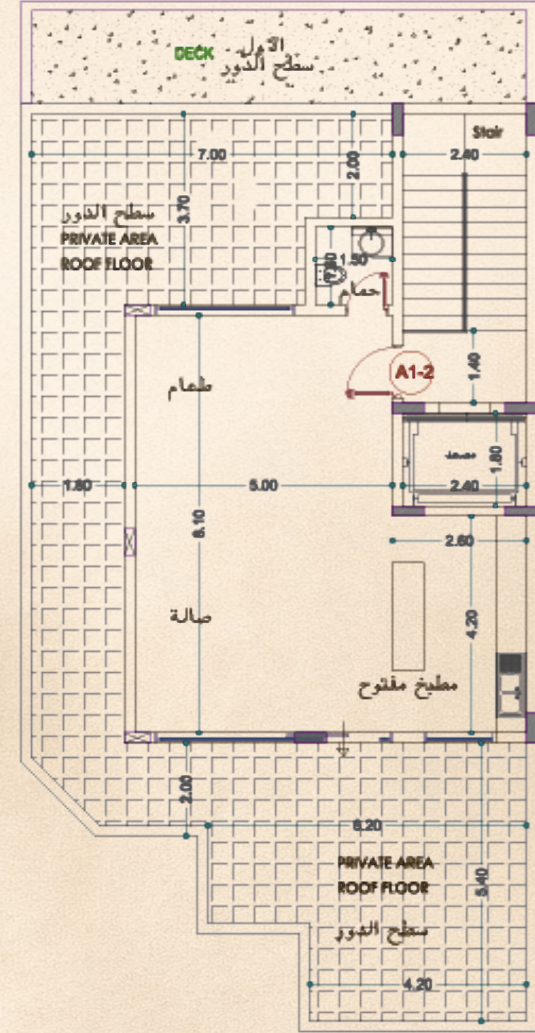
AI-2 ROOF FLOOR PLAN
