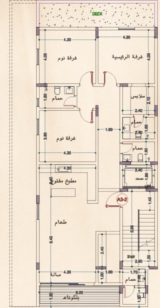
A3-2 FIRST FLOOR PLAN
